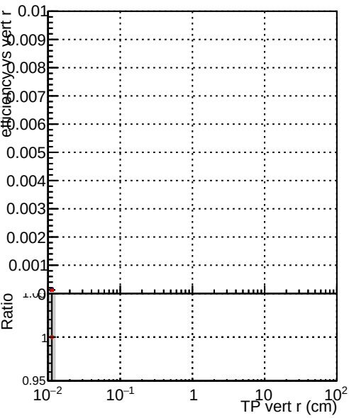
Efficiency vs vertpos Legend: DQM_V0001_R0000000001_Global_mkFitNewOLD1000time_RECO DQM_V0001_R0000000001_Global_mkFitOLD-checkDet12_RECO
