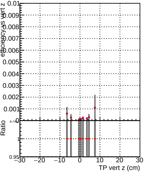
Efficiency vs vertpos Legend: DQM_V0001_R0000000001_Global_mkFitNewOLD1000time_RECO DQM_V0001_R0000000001_Global_mkFitOLD-checkDet12_RECO
