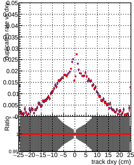
al_mkFitNewOLD1000time__RECO al_mkFitOLD-checkDet12__RECO
