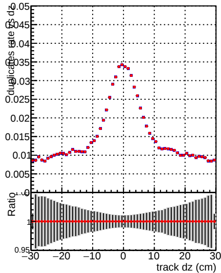
al_mkFitNewOLD1000time__RECO al_mkFitOLD-checkDet12__RECO
