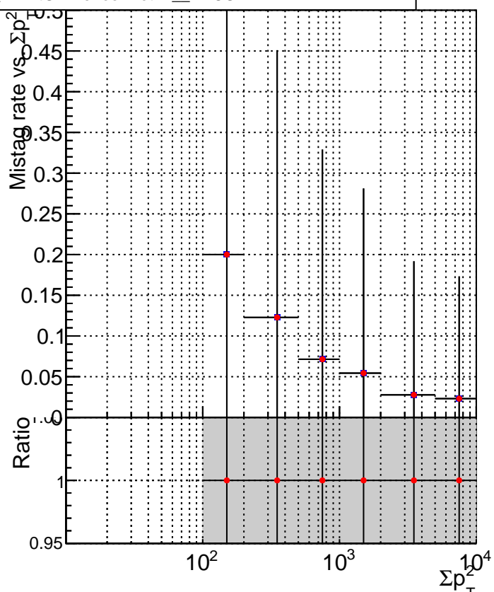
■ DQM_V0001_R000000001_Global_mkFitNewOLD1000time_RECO ● DQM_V0001_R000000001_Global_mkFitOLD-checkDet12_RECO
