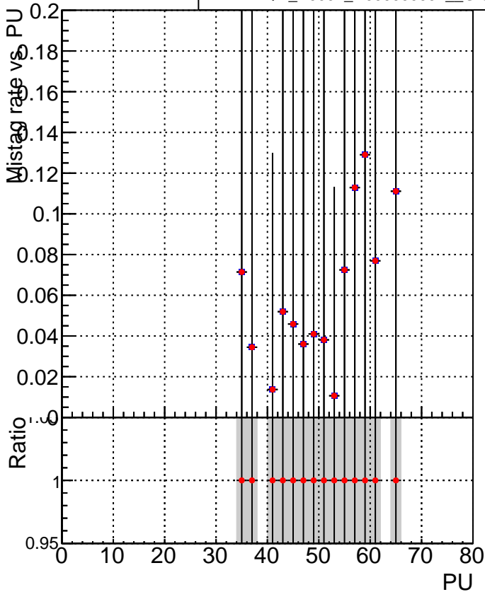
■ DQM_V0001_R000000001_Global_mkFitNewOLD1000time_RECO ● DQM_V0001_R000000001_Global_mkFitOLD-checkDet12_RECO
