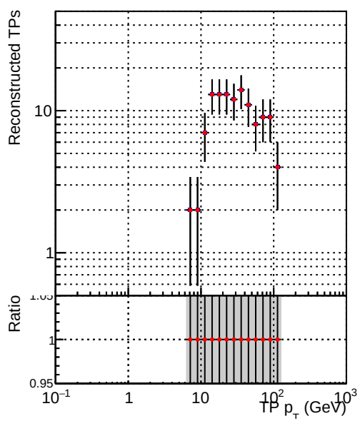
—●— DQM_V0001_R0000000001_Global_mkFitNewOLD1000time_RECO —●— DQM_V0001_R0000000001_Global_mkFitOLD-checkDet12_RECO
