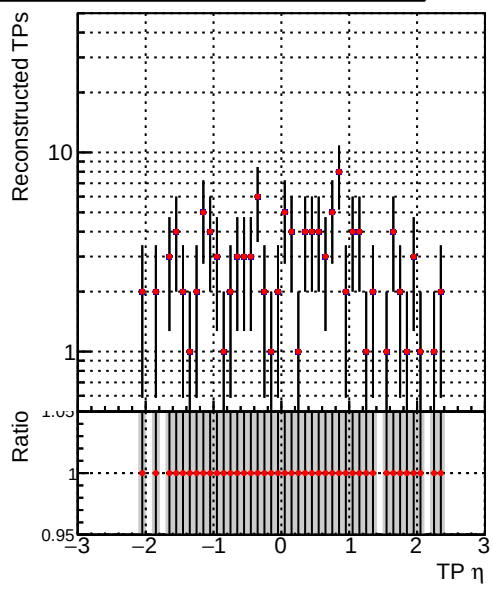
—●— DQM_V0001_R0000000001_Global_mkFitNewOLD1000time_RECO —●— DQM_V0001_R0000000001_Global_mkFitOLD-checkDet12_RECO
