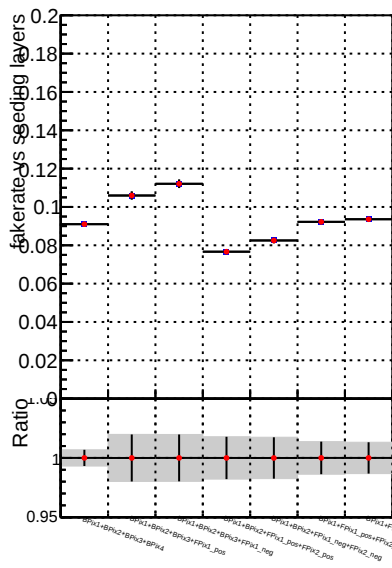
Fake rate vs. —●— DQM_V0001_R0000000001 Global mkFitNewOLD1000time RECO —●— DQM_V0001_R0000000001 Global mkFitOLD-checkDet12 RECO
