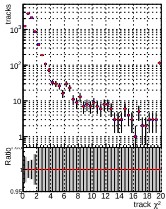
N of reco track vs. —●— DQM_V0001_R000000001_Global_mkFitNewOLD1000time_RECO —●— DQM_V0001_R000000001_Global_mkFitOLD-checkDet12_RECO
