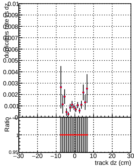
Global mkFitNewOLD1000time RECO Global mkFitOLD-checkDet12 RECO
