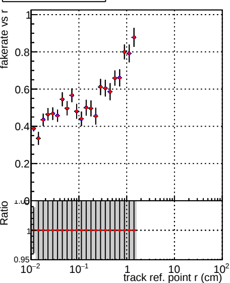
Legend: —●— DQM_V0001_R000000001_Global_mkFitNewOLD1000time_RECO —●— DQM_V0001_R000000001_Global_mkFitOLD-checkDet12_RECO
