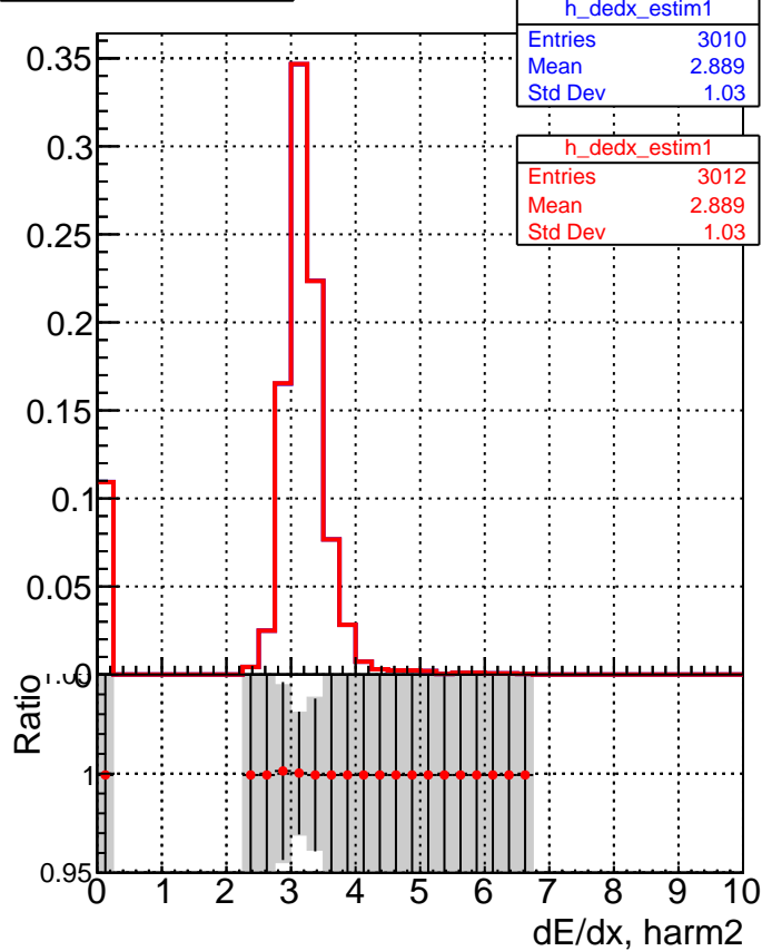
■ DQM_V0001_R000000001_Global_mkFitNewOLD1000time_RECO ● DQM_V0001_R000000001_Global_mkFitOLD-checkDet12_RECO
