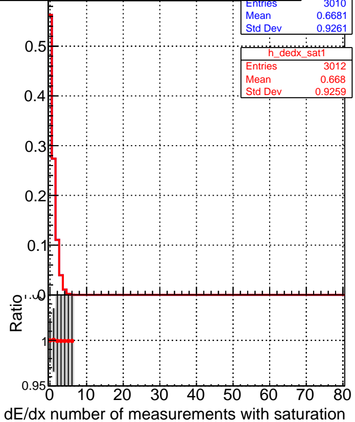
■ DQM_V0001_R000000001_Global_mkFitNewOLD1000time_RECO ● DQM_V0001_R000000001_Global_mkFitOLD-checkDet12_RECO
