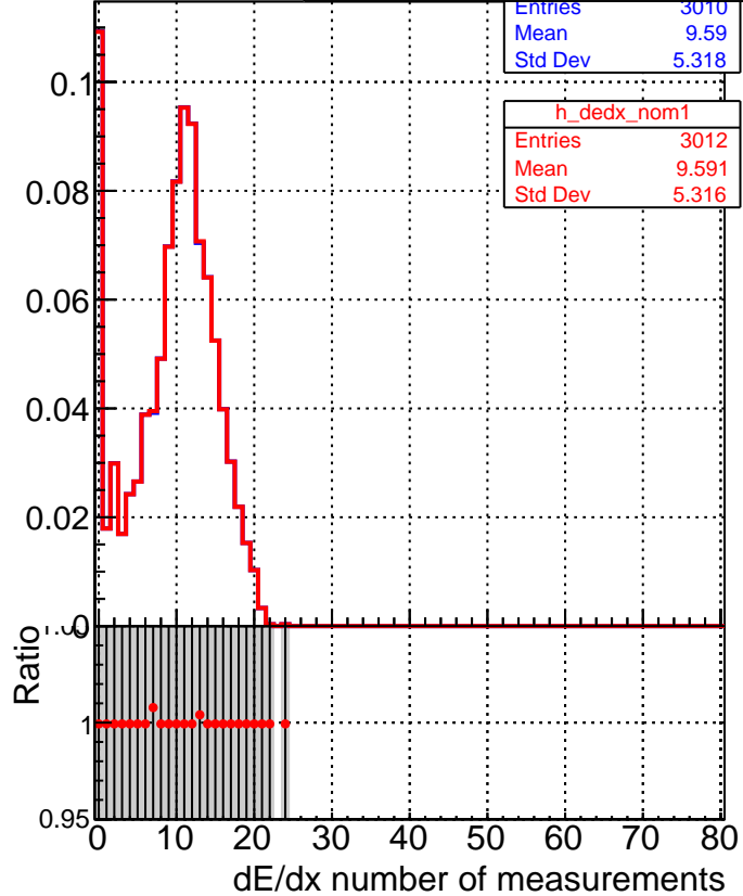
■ DQM_V0001_R000000001_Global_mkFitNewOLD1000time_RECO ● DQM_V0001_R000000001_Global_mkFitOLD-checkDet12_RECO
