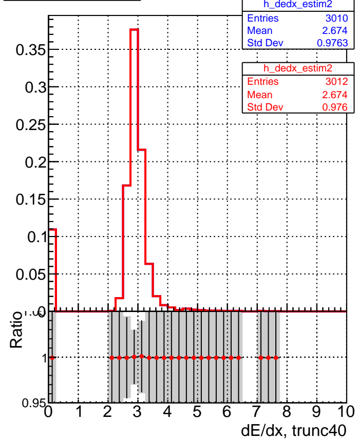
■ DQM_V0001_R000000001_Global_mkFitNewOLD1000time_RECO ● DQM_V0001_R000000001_Global_mkFitOLD-checkDet12_RECO
