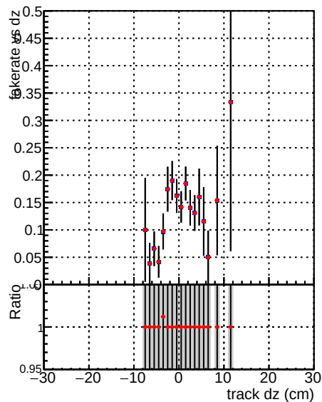
Fake rate vs dz DQM V0001_R000000001 Global mkFitNewOLD1000time RECO DQM V0001_R000000001 Global mkFitOLD-checkDet12 RECO
