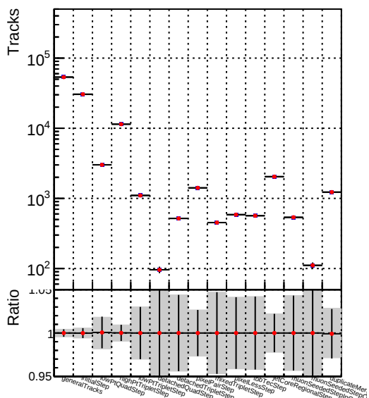
DQM_V0001_R000000001_Global_mkFitNewOLD1000time_RECO
