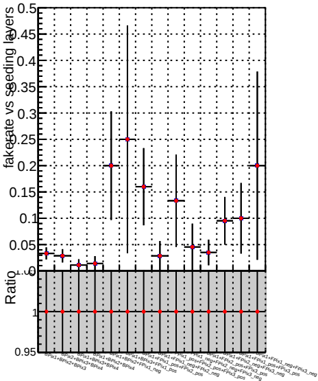
Fake rate vs. — DQM_V0001_R000000001 Global mkFitNewOLD1000time RECO — DQM_V0001_R000000001 Global mkFitOLD-checkDet12 RECO
