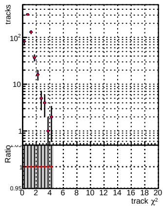
N of reco track vs. \chi^2 — Global mkFitNewOLD1000time RECO — Global mkFitOLD-checkDet12 RECO
