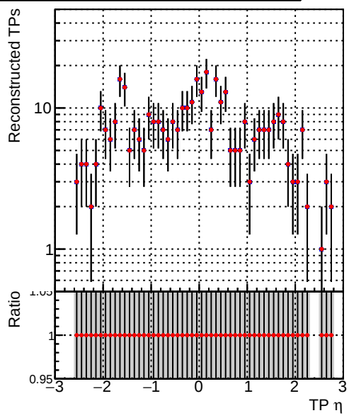
Legend: DQM_V0001_R000000001_Global_mkFitNewOLD1000time_RECO (blue line), DQM_V0001_R000000001_Global_mkFitOLD-checkDet12_RECO (red line)
