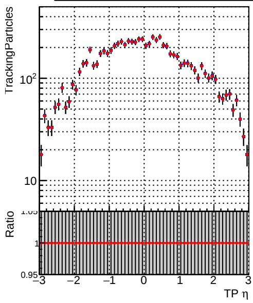
Legend: DQM_V0001_R000000001_Global_mkFitNewOLD1000time_RECO (blue line), DQM_V0001_R000000001_Global_mkFitOLD-checkDet12_RECO (red line)
