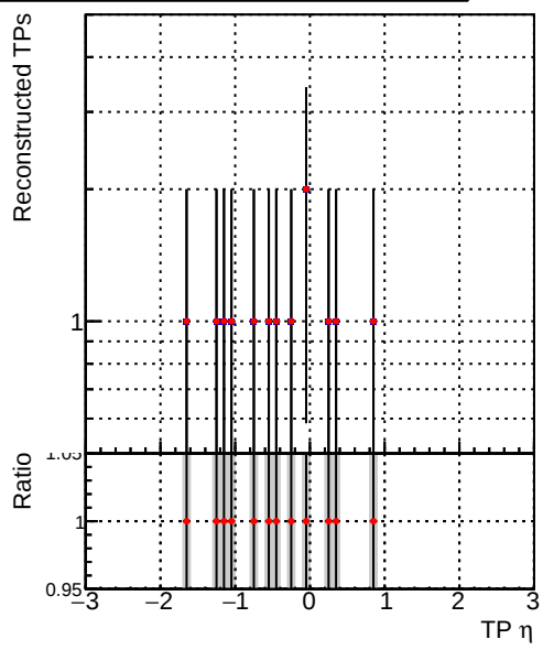
—●— DQM_V0001_R000000001_Global_mkFitNewOLD1000time_RECO —●— DQM_V0001_R000000001_Global_mkFitOLD-checkDet12_RECO
