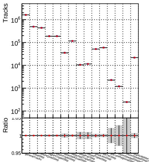
DQM_V0001_R000000001_Global_mkFitNewOLD1000time_RECO
