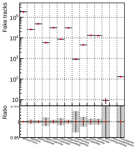
Number —●— DQM_V0001_R000000001_Global_mkFitOLD-checkDet12_RECO
