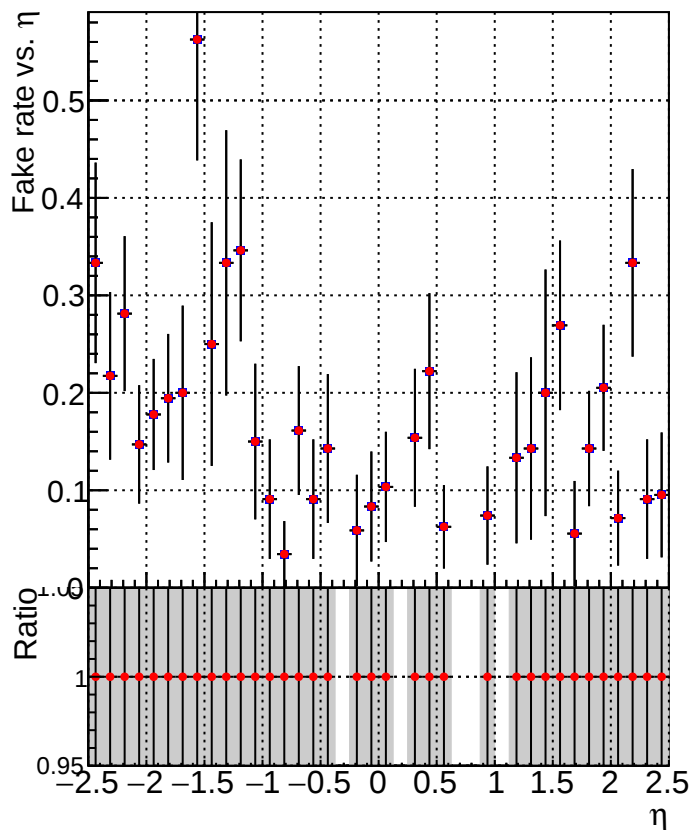
\Lambda tracking fake rate vs \eta
