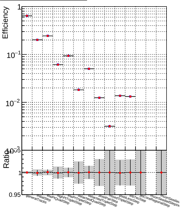
DQM_V0001_R000000001_Global_mkFitOLD_RECO DQM_V0001_R000000001_Global_mkFitNEW_RECO
