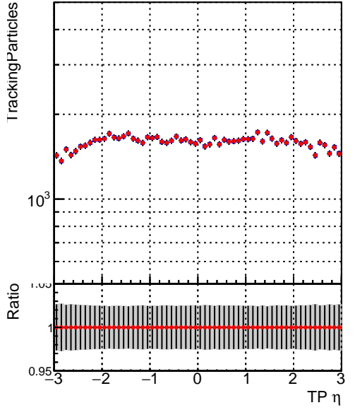
█ DQM_V0001_R000000001_Global_mkFitOLD_RECO █ DQM_V0001_R000000001_Global_mkFitNEW_RECO
