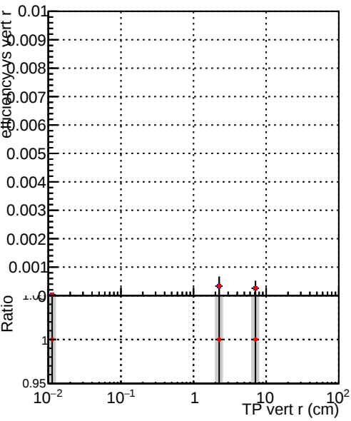
Efficiency vs vertpos Legend: DQM_V0001_R000000001_Global_mkFitOLD_RECO DQM_V0001_R000000001_Global_mkFitNEW_RECO
