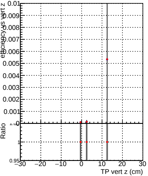
Efficiency vs vertpos Legend: DQM_V0001_R000000001_Global_mkFitOLD_RECO DQM_V0001_R000000001_Global_mkFitNEW_RECO
