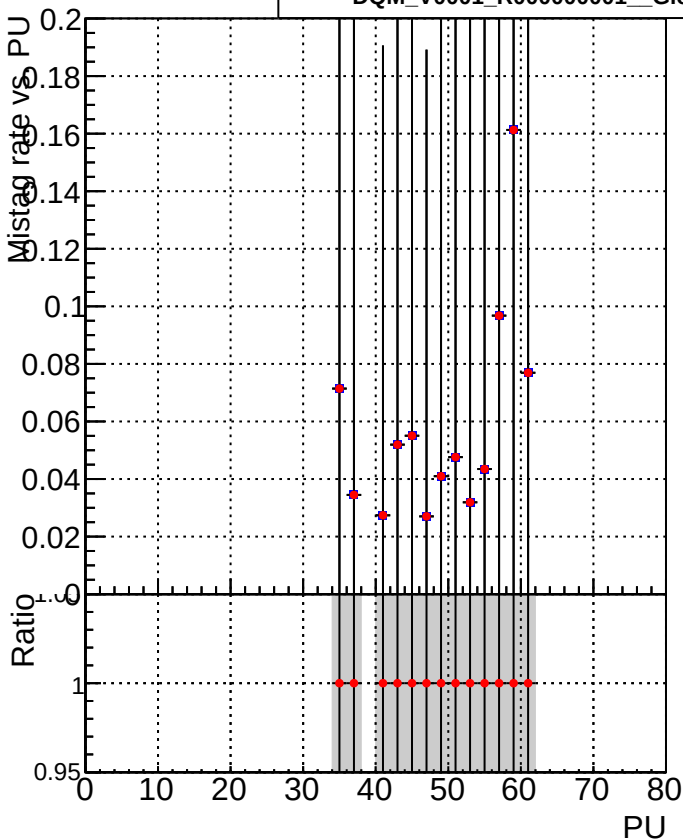
DQM_V0001_R000000001_Global_mkFitOLD_RECO DQM_V0001_R000000001_Global_mkFitNEW_RECO
