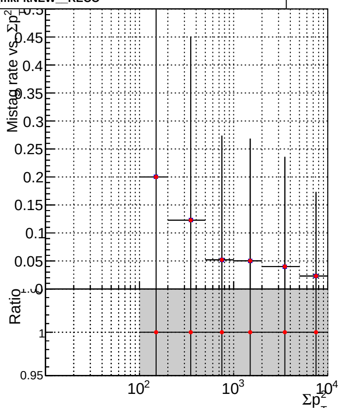
DQM_V0001_R000000001_Global_mkFitOLD_RECO DQM_V0001_R000000001_Global_mkFitNEW_RECO
