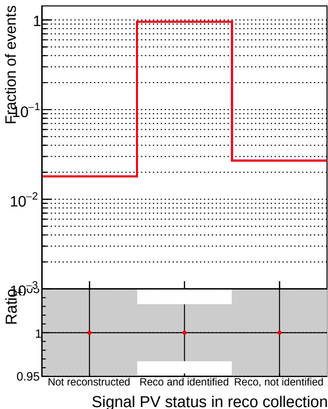
DQM_V0001_R000000001_Global_mkFitOLD_RECO DQM_V0001_R000000001_Global_mkFitNEW_RECO
