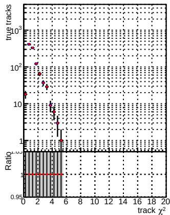
DOM_V0001_R000000001_Global_mkFitOLD_RECO DOM_V0001_R000000001_Global_mkFitNEW_RECO
