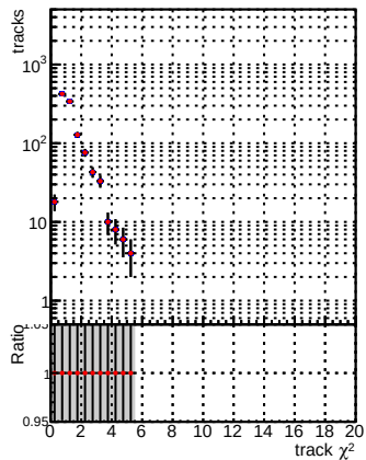
DOM_V0001_R000000001_Global_mkFitOLD_RECO DOM_V0001_R000000001_Global_mkFitNEW_RECO
