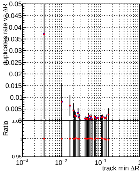
—●— DQM_V0001_R000000001_Global_mkFitOLD_RECO —●— DQM_V0001_R000000001_Global_mkFitNEW_RECO
