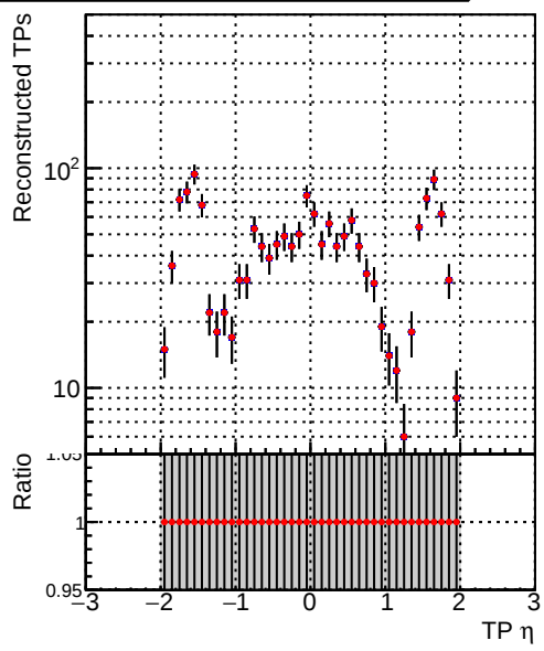
— DQM_V0001_R000000001_Global_mkFitOLD_RECO — DQM_V0001_R000000001_Global_mkFitNEW_RECO
