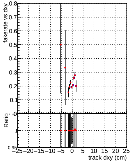
DQM_V0001_R0000000001 Global mkFitOLD RECO Fake rate vs d
