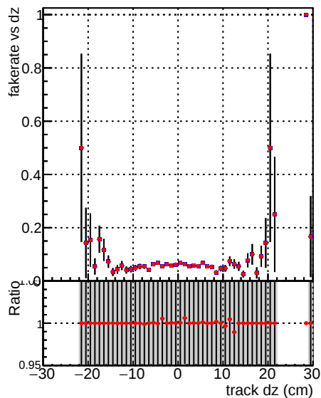
Fake rate vs dz DQM_V0001_R0000000001 Global mkFitOLD RECO Duplicates Rate vs Dxy DQM_V0001_R0000000001 Global mkFitNEW RECO
