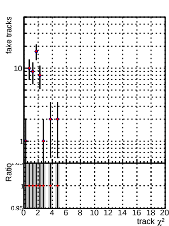
Legend: - Blue line: DQM_V0001_R0000000001_Global_mkFitOLD_RECO - Red line: DQM_V0001_R0000000001_Global_mkFitNEW_RECO
