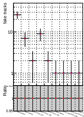
Legend: - Blue line: DQM_V0001_R0000000001_Global_mkFitOLD_RECO - Red line: DQM_V0001_R0000000001_Global_mkFitNEW_RECO
