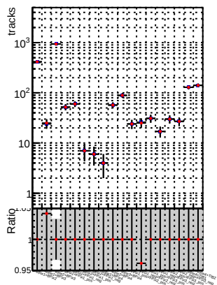
Legend: - Blue line: DQM_V0001_R0000000001_Global_mkFitOLD_RECO - Red line: DQM_V0001_R0000000001_Global_mkFitNEW_RECO
