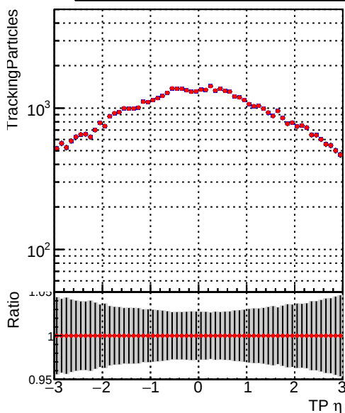
— DQM_V0001_R000000001_Global_mkFitOLD_RECO — DQM_V0001_R000000001_Global_mkFitNEW_RECO
