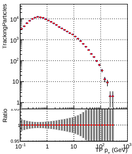
— DQM_V0001_R000000001_Global_mkFitOLD_RECO — DQM_V0001_R000000001_Global_mkFitNEW_RECO
