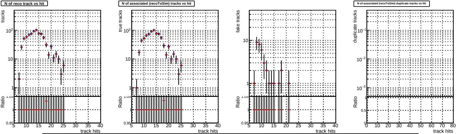
DQM_V0001_R000000001_Global_mkFitOLD_RECO DQM_V0001_R000000001_Global_mkFitNEW_RECO
