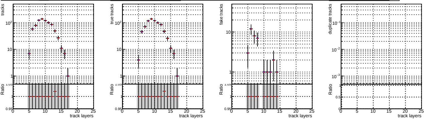
DQM_V0001_R000000001_Global_mkFitOLD_RECO DQM_V0001_R000000001_Global_mkFitNEW_RECO
