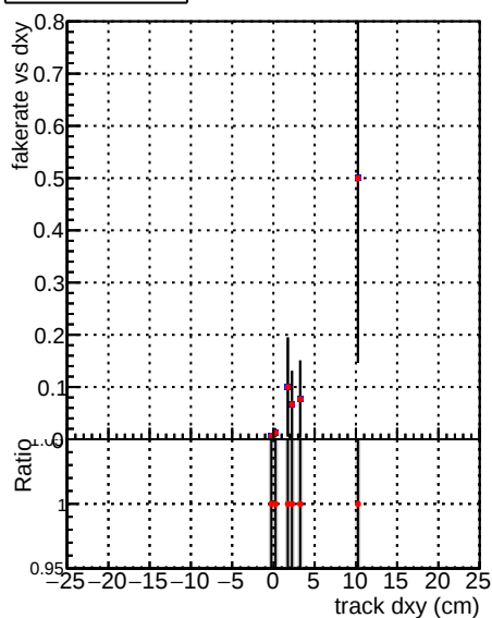
Global mkFitOLD RECO Fake rate vs d DQM V0001_R000000001 DQM V0001_R000000001 DQM V0001_R000000001 Duplicates Rate vs Dxy DQM V0001_R000000001 DQM V0001_R000000001 DQM V0001_R000000001 Pileup rate vs dxy DQM V0001_R000000001 DQM V0001_R000000001 DQM V0001_R000000001 Fake rate vs dz DQM V0001_R000000001 DQM V0001_R000000001 DQM V0001_R000000001 Duplicates Rate vs Dxy DQM V0001_R000000001 DQM V0001_R000000001 DQM V0001_R000000001 Pileup rate vs dz DQM V0001_R000000001 DQM V0001_R000000001 DQM V0001_R000000001
