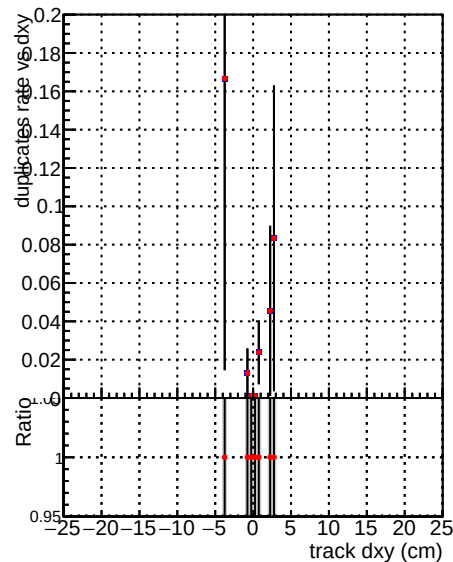
al__mkFitOLD__RECO al__mkFitNEW__RECO
