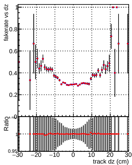
Fake rate vs dz —●— DQM_V0001_R0000000001 Global mkFitOLD RECO —●— DQM_V0001_R0000000001 Global mkFitNEW RECO
