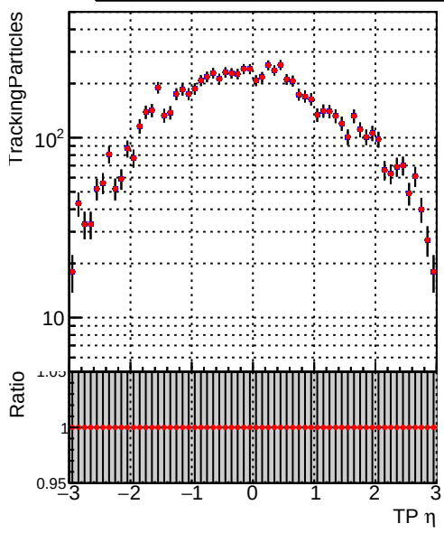
Legend: DQM_V0001_R000000001_Global_mkFitOLD_RECO (blue line), DQM_V0001_R000000001_Global_mkFitNEW_RECO (red line)
