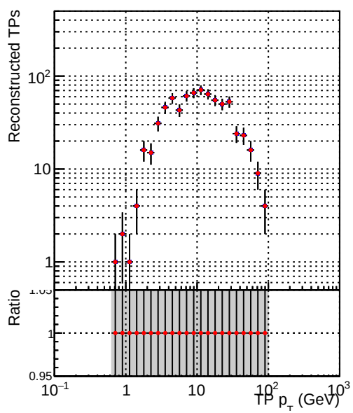
Legend: DQM_V0001_R000000001_Global_mkFitOLD_RECO (blue line), DQM_V0001_R000000001_Global_mkFitNEW_RECO (red line)
