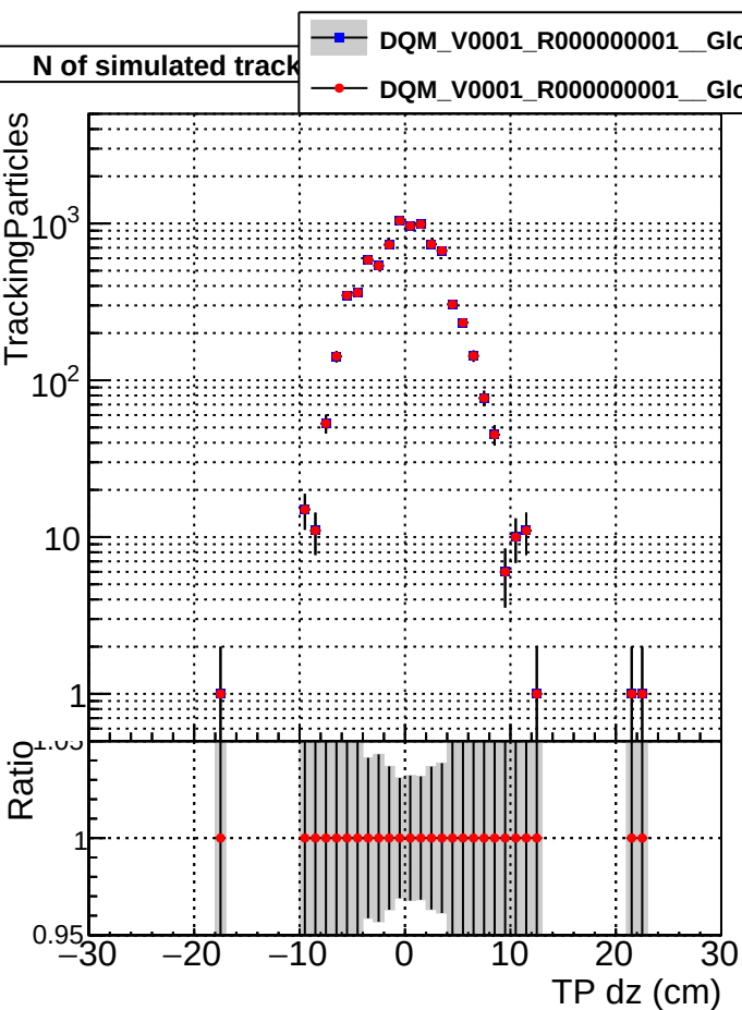
DQM_V0001_R000000001_Global_mkFitOLD_RECO
