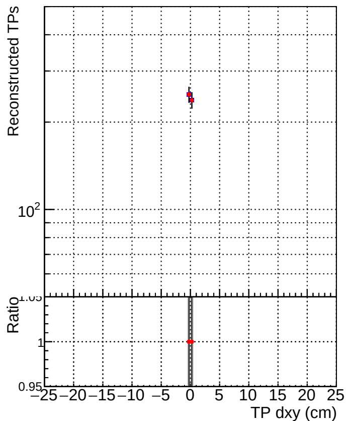
DQM_V0001_R000000001_Global_mkFitOLD_RECO
