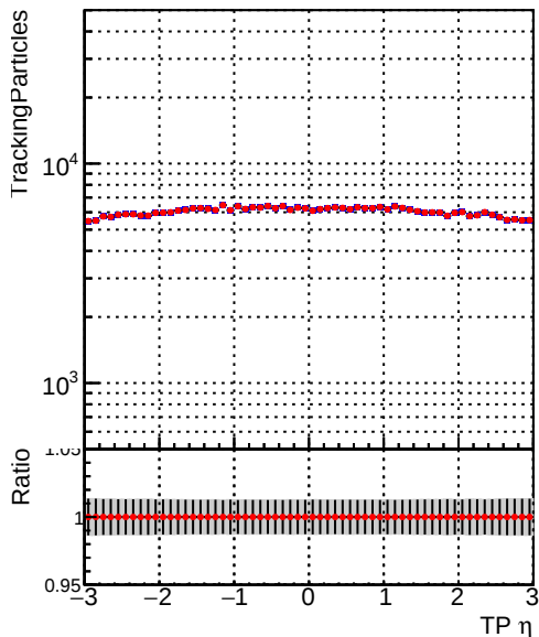
DQM_V0001_R000000001_Global_mkFitOLD_RECO DQM_V0001_R000000001_Global_mkFitNEW_RECO
