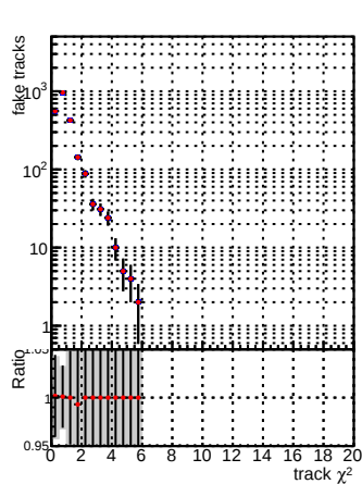
Legend: - Blue line: DQM_V0001_R0000000001_Global_mkFitOLD_RECO - Red line: DQM_V0001_R0000000001_Global_mkFitNEW_RECO - Grey bar: verSet
