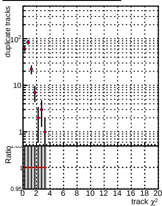
Legend: - Blue line: DQM_V0001_R0000000001_Global_mkFitOLD_RECO - Red line: DQM_V0001_R0000000001_Global_mkFitNEW_RECO - Grey bar: verSet
