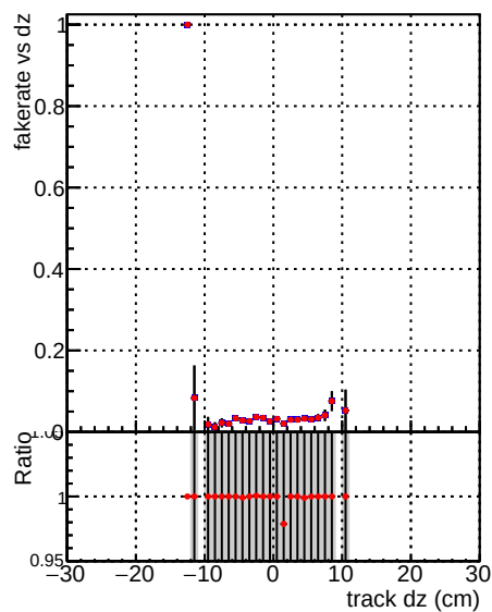
Fake rate vs dz DQM V0001_R0000000001 Global mkFitOLD RECO
