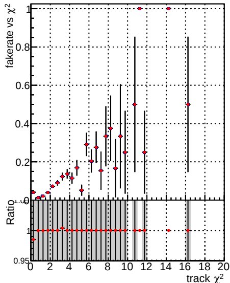
—●— DQM_V0001_R0000000001_Global_mkFitOLD_RECO —●— DQM_V0001_R0000000001_Global_mkFitNEW_RECO
