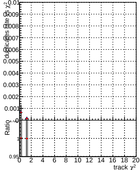
—●— DQM_V0001_R0000000001_Global_mkFitOLD_RECO —●— DQM_V0001_R0000000001_Global_mkFitNEW_RECO
