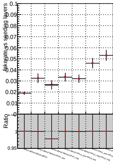
—●— DQM_V0001_R0000000001_Global_mkFitOLD_RECO —●— DQM_V0001_R0000000001_Global_mkFitNEW_RECO
