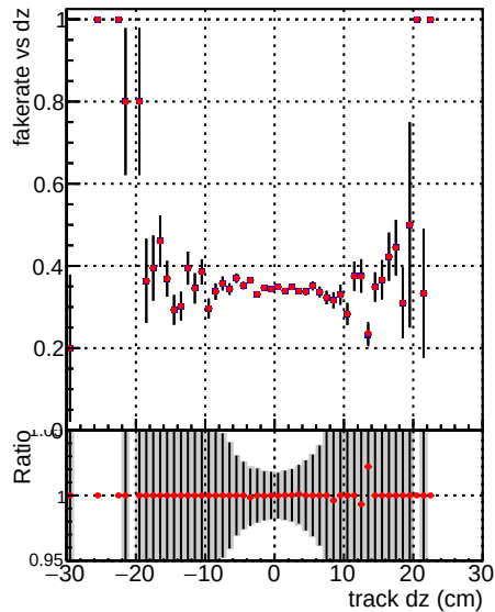
Fake rate vs d DQM V0001_R000000001 Global mkFitOLD RECO DQM V0001_R000000001 Global mkFitNEW RECO
