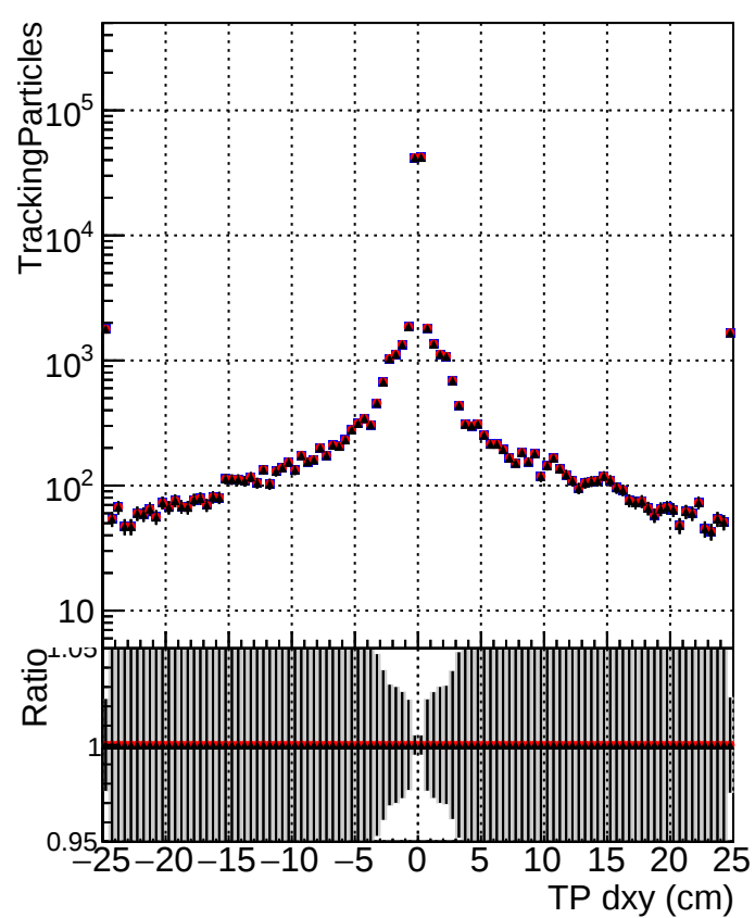
N of simulated track ■ DQM_V0001_R000000001 Global CMSSW_ckftt502_RECO ● DQM_V0001_R000000001 Global CMSSW_mkttt502_RECO ▲ DQM_V0001_R000000001 Global CMSSW_mkttt50i3_RECO
