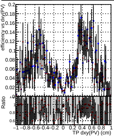
Efficiency vs Dxy(PV) Legend: DQM_V0001_R000000001_Global_CMSSW_ckpt502_RECO DQM_V0001_R000000001_Global_CMSSW_mkt502_RECO DQM_V0001_R000000001_Global_CMSSW_mkt50i3_RECO
