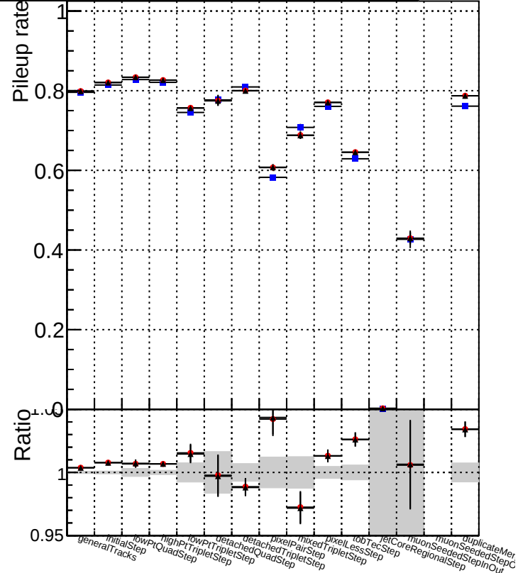
■ DQM_V0001_R000000001 Global CMSSW ckftt502 RECO ● DQM_V0001_R000000001 Global CMSSW mkt502 RECO ▲ DQM_V0001_R000000001 Global CMSSW mkt503 RECO
