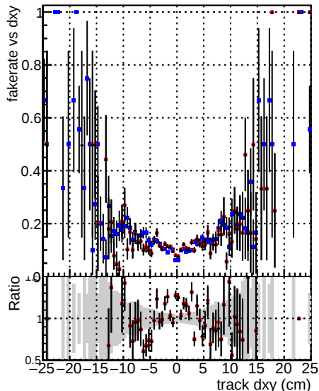
DOM V0001 RECO Global V0001 RECO CMSSW ckt502 RECO DOM V0001 RECO Global V0001 RECO CMSSW mkt503 RECO
