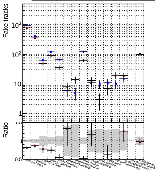
Number Legend Series Name DQM_V0001_R0000000001_Global_CMSSW_ckftt502_RECO DQM_V0001_R0000000001_Global_CMSSW_mkttt502_RECO DQM_V0001_R0000000001_Global_CMSSW_mkttt503_RECO
