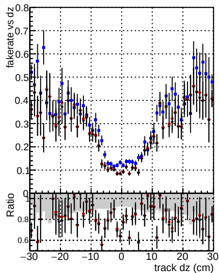
DOM V0001 DOM V0001 RECO Global CMSSW ckft502 RECO DOM V0001 DOM V0001 RECO Global CMSSW mkt502 RECO DOM V0001 DOM V0001 RECO Global CMSSW mkt503 RECO
