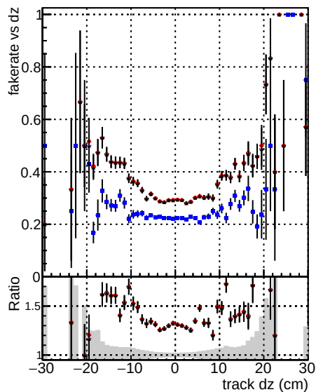
DOM V0001 DOM V0001 RECO Global V0001 RECO CMSSW ckt502 RECO DOM V0001 DOM V0001 RECO Global V0001 RECO CMSSW mkt503 RECO
