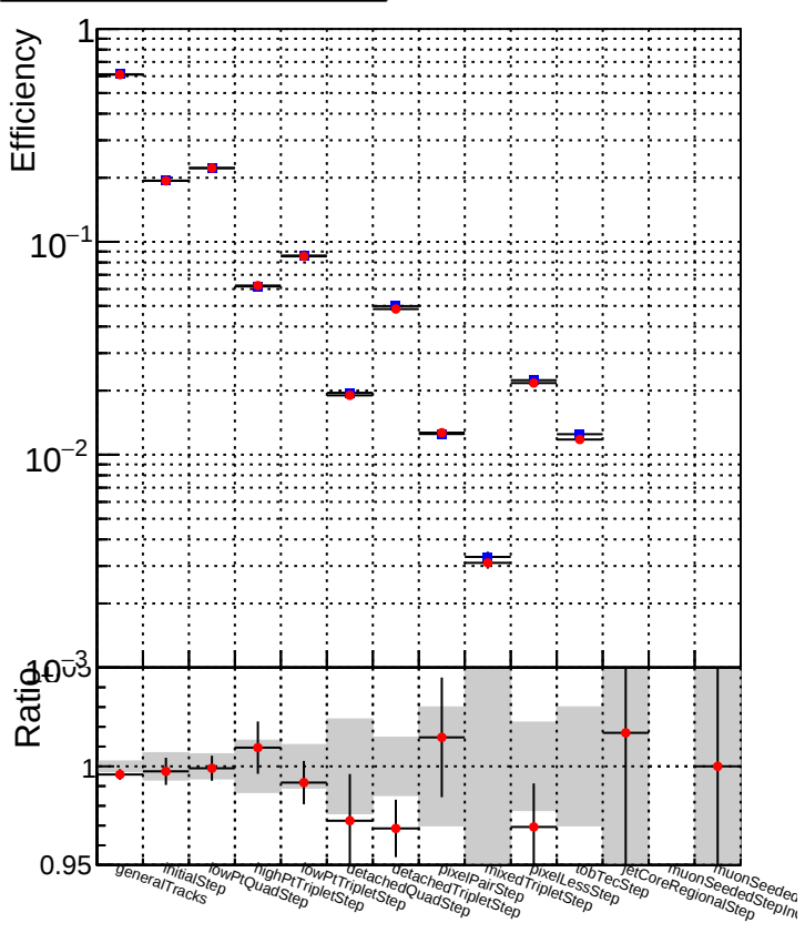
DQM_mkFit_TToriginal DQM_mkFit_TTNEWnoMS-genMatch-CUT
