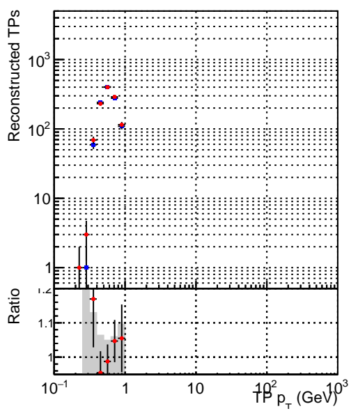
—•— DQM_mkFit_TToriginal —•— DQM_mkFit_TTNEWnoMS-genMatch-CUT
