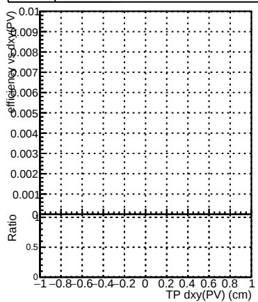
Efficienc ● DQM_mkFit_TTNEWnoMS-genMatch-CUT
